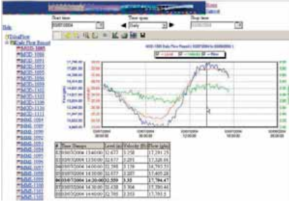
Real-time DAS data presentation via web browser.
